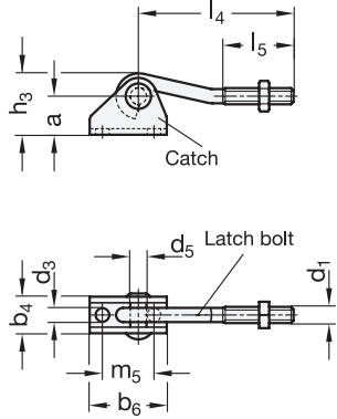
Type TU J-hook latch bolt
