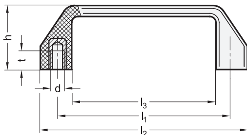
GN 528.1
